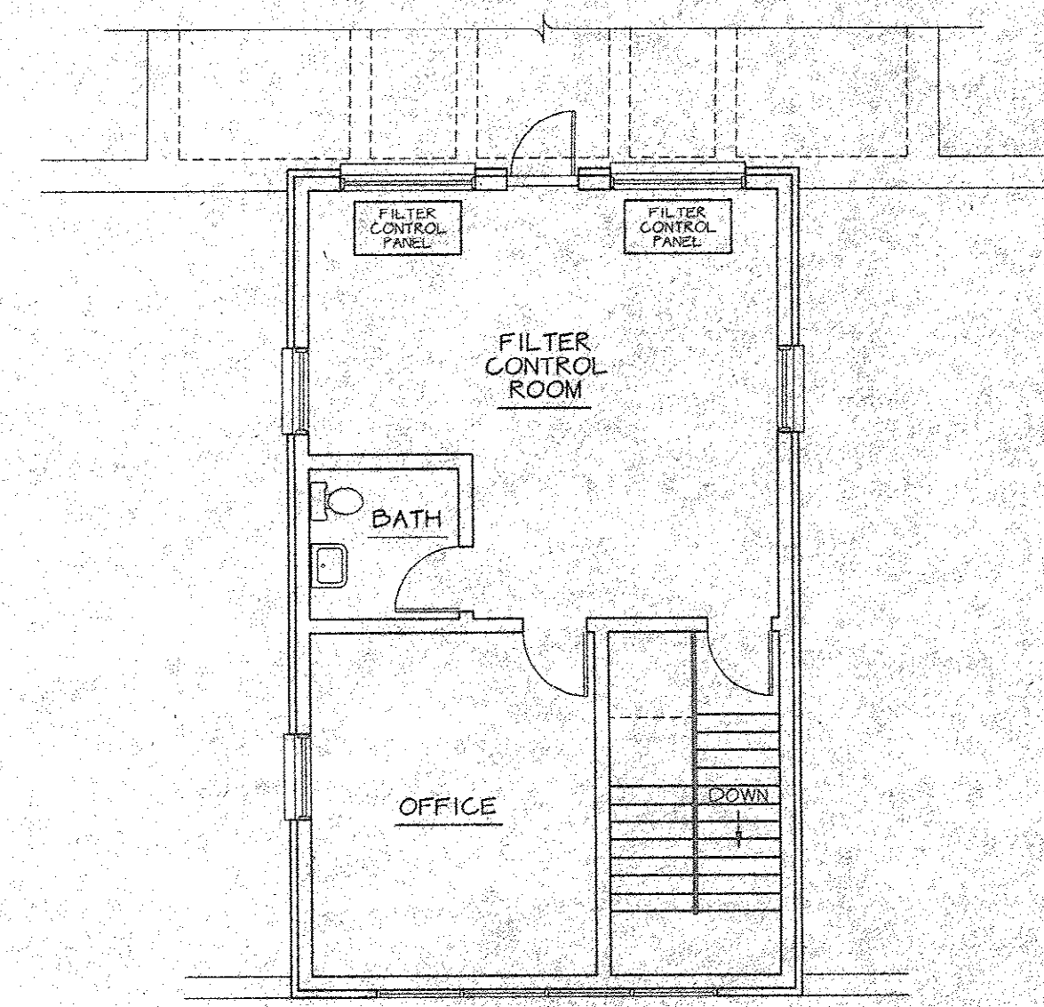
SECOND FLOOR PLAN SCALE: 1/8" = 1'-0"
