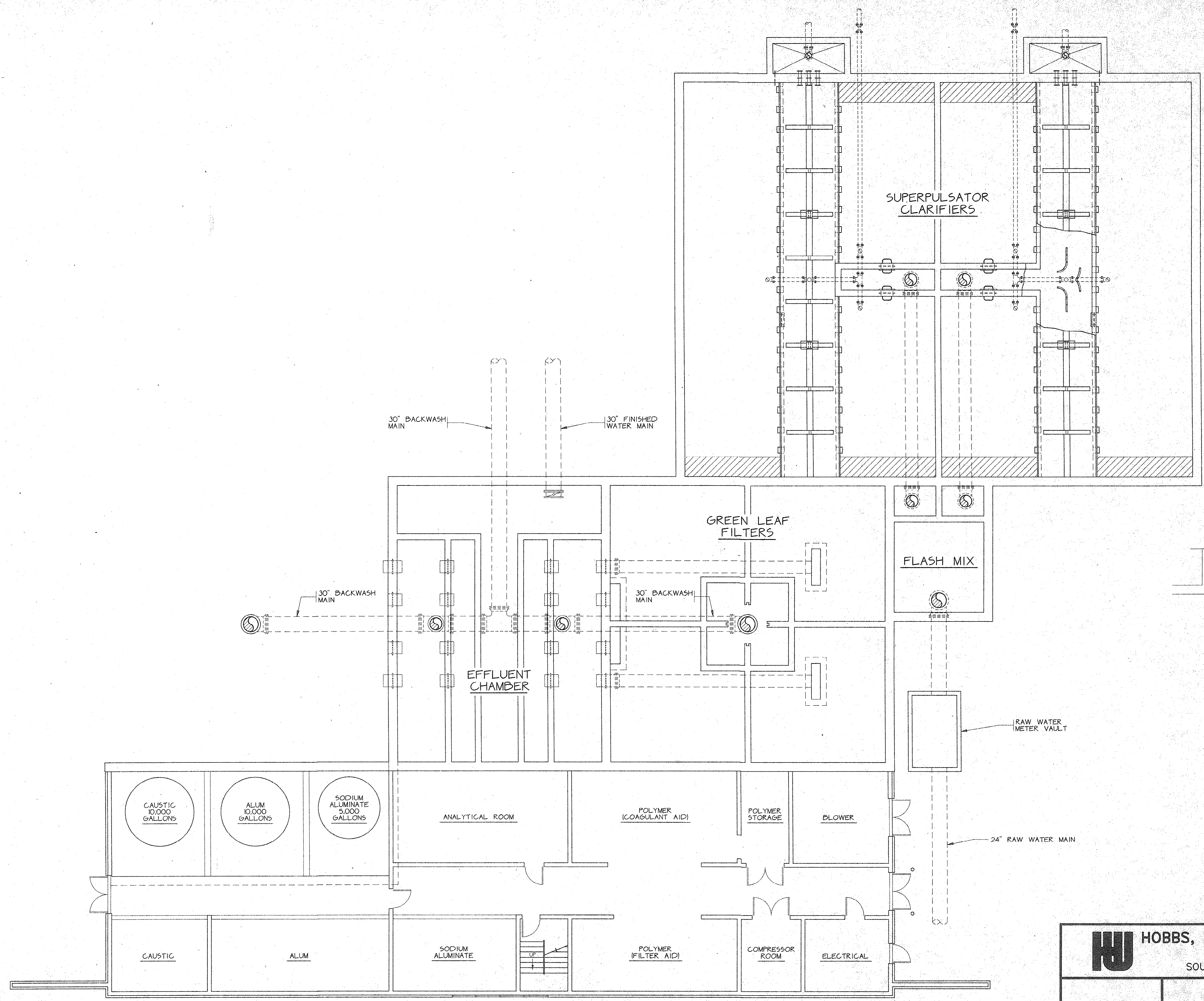
PLANT UNIT LAYOUT LOWER FLOOR PLAN SCALE: 1/8" = 1'-0"
